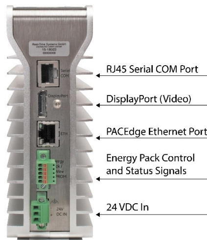
Figure 3: Underside Ports & Connectors
