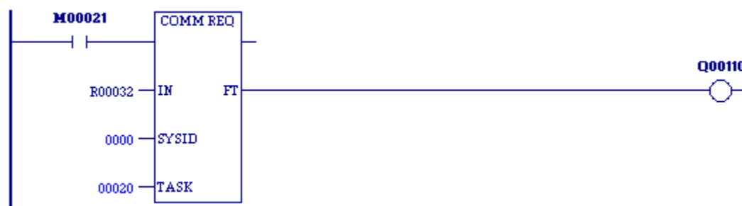
Figure 35: COMMREQ Example
