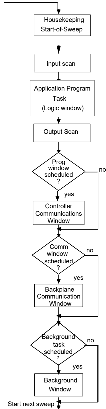
Figure 26: Major Phases of a Typical CPU Sweep
