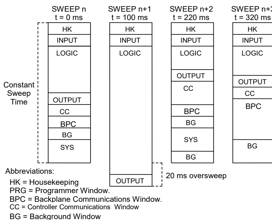
Figure 28: Typical Sweeps in Constant Sweep Mode
