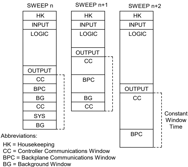
Figure 29: Typical Sweeps in Constant Window Mode
