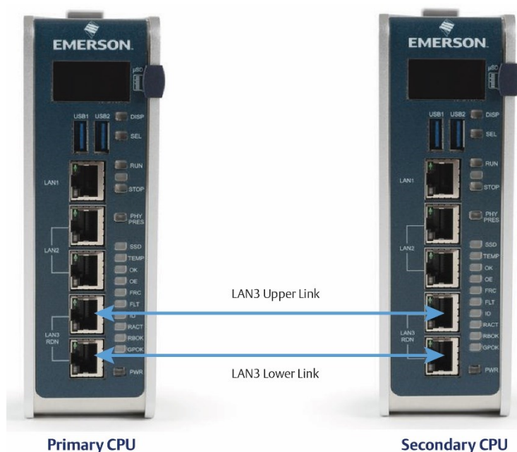
Figure 6: LAN3 Interconnects for Hot Standby Redundancy
