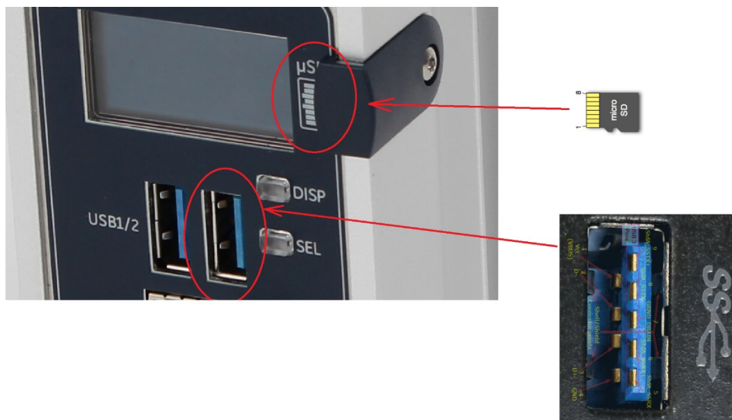
Figure 4: CPE400 Micro-SD & USB Connectors
