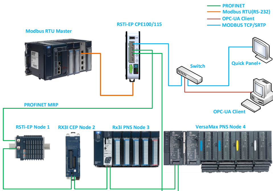
Figure 22: Typical Multi-Tier LAN Application (Star/Bus Topology)
