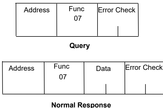
Figure 45: RTU Read Exception Status Message Format
