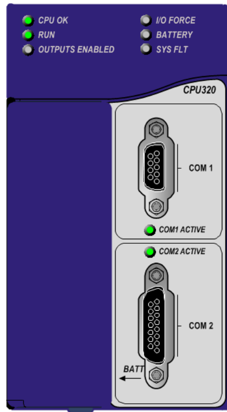
Figure 17: IC695CPU320 Front View
