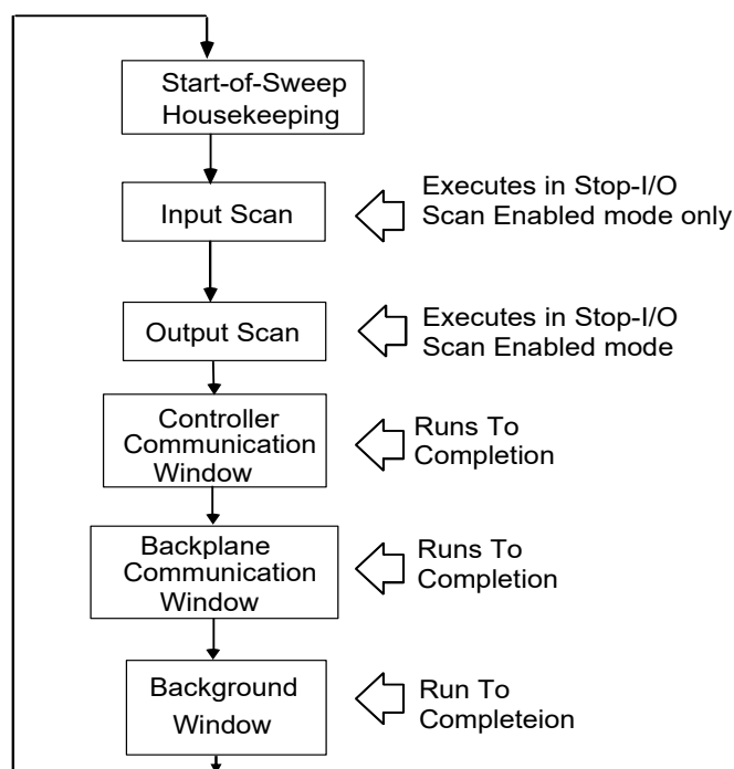
Figure 30: CPU Sweep in Stop-I/O Disabled and Stop-I/O Enabled Modes
