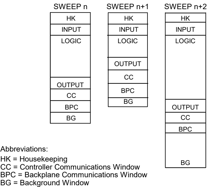
Figure 27: Typical Sweeps in Normal Sweep Mode
