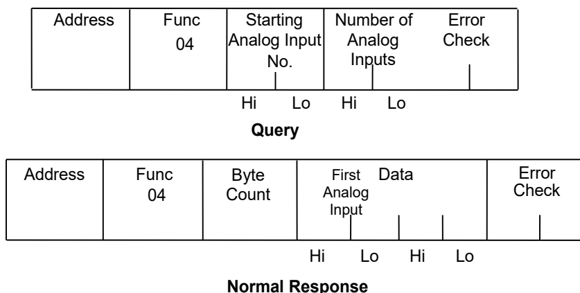
Figure 42: RTU Read Analog Inputs Message Format
