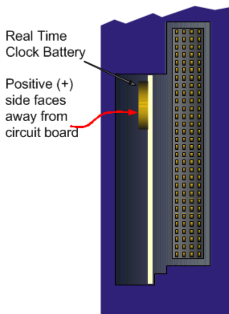
Figure 15: Accessing Real-Time Clock Battery (CPE302, CPE305, and CPE310)
