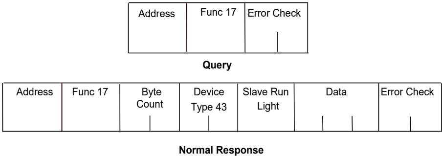
Figure 49: RTU Report Device Type Message Format
