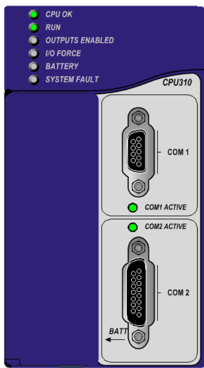
Figure 18: CPU310 Front View
