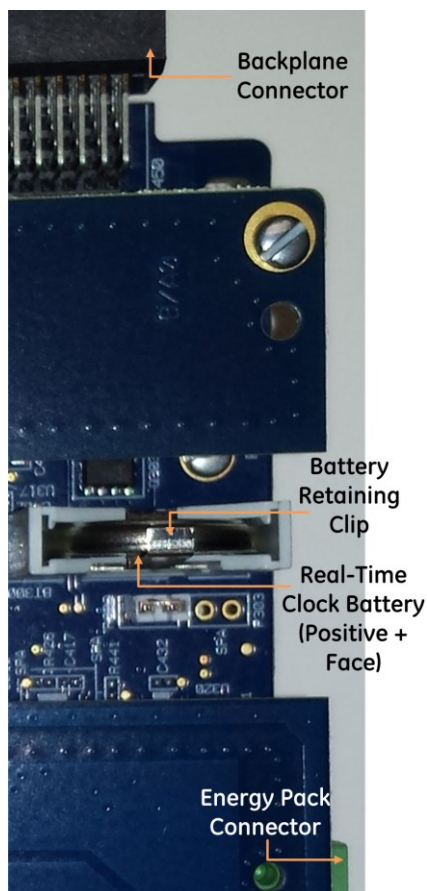
Figure 10: Location and Orientation of Real-Time Clock Battery in CPE330
