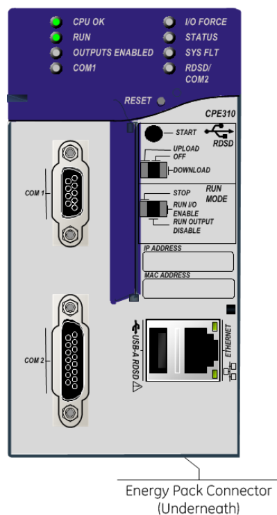
Figure 14: External Features of CPE310
